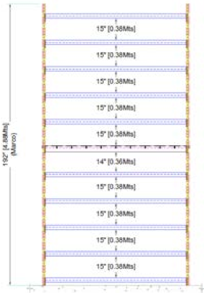
VISTA FRONTAL RACK SELECTIVO
